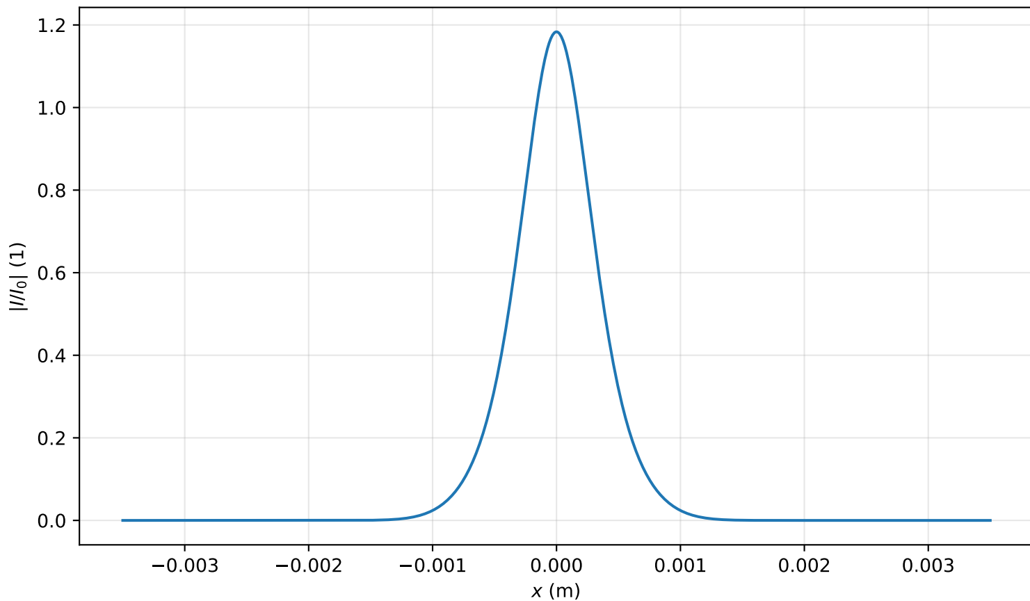
Intensity profile I(x, y = 0, z = 0.876m)/I_0 , P_{in}=0.7P_{cr} , artificial time
